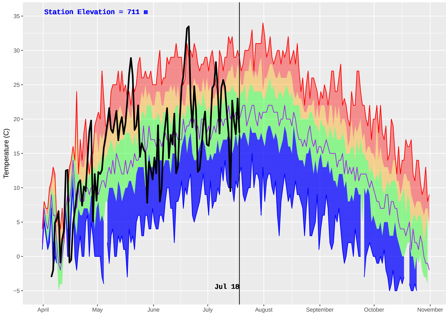
TOAD RIVER (126) : Historical (1981–2016) and Current (2018) Daily Temperature
